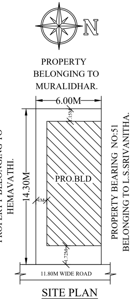
SITE PLAN
